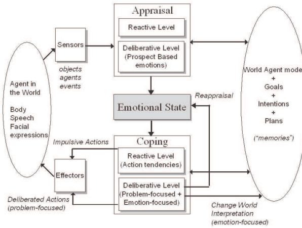
Fig. 2. Architecture Diagram
