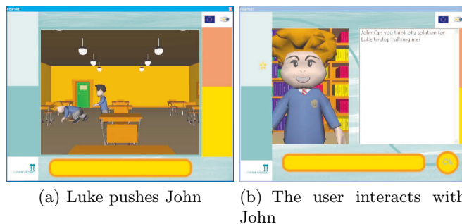
Fig. 1. FearNot! application
